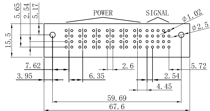
P.C. Body Hole Layout
